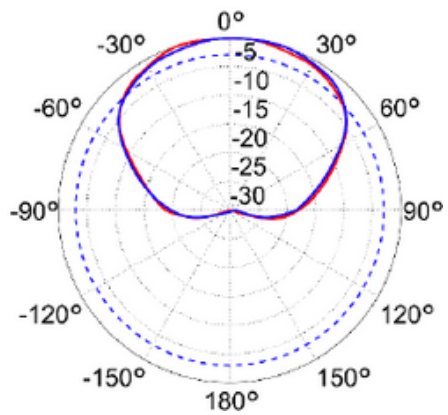
Azimuth Pattern
