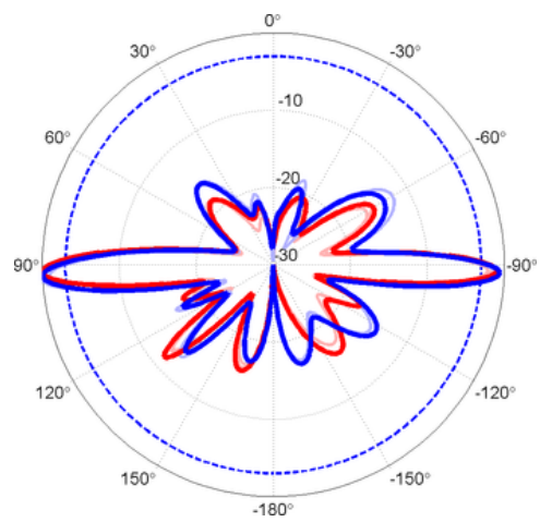
Gain
