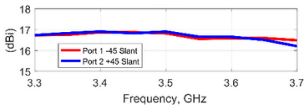
Gain
